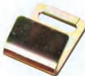
HYFH-078 A=48mm B=92mm C=4.5mm PULL ≤ 5000KG
